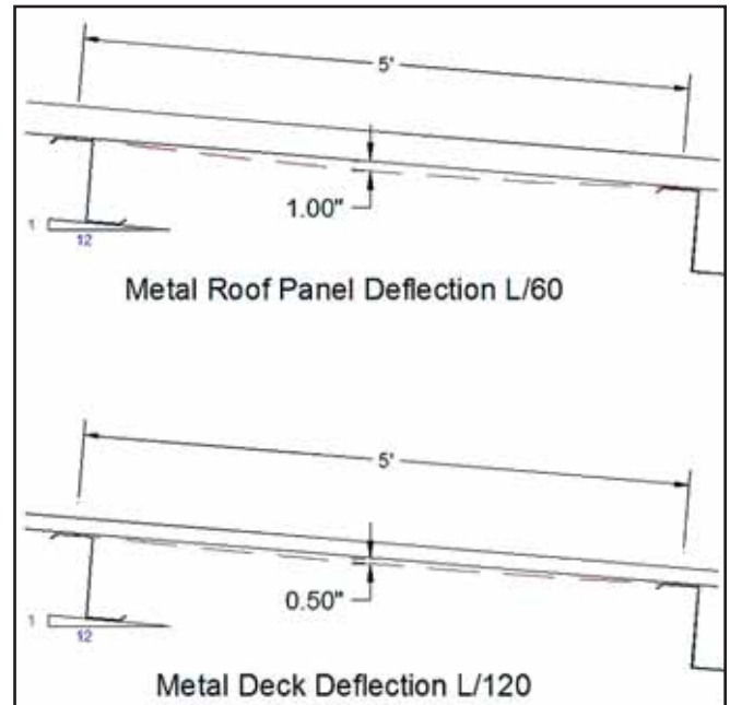
6. Metal roof and metal decking deflection comparisons.
