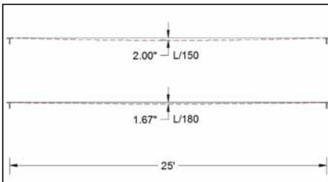
5. Secondary structural member deflection limits at a 25-foot span.
