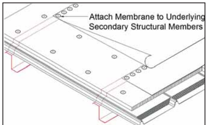
12. Single-ply roof fastening to underlying secondary members.
