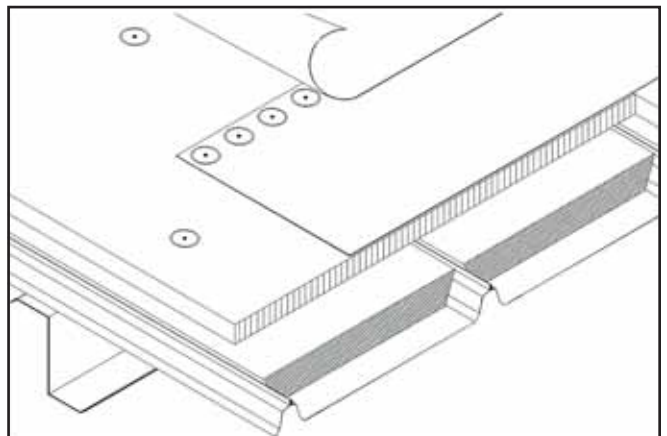
2. Example of a single-ply over metal retrofit assembly.
