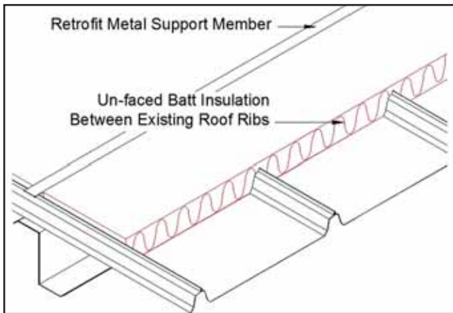
14. One example of metal roof retrofit insulation.
