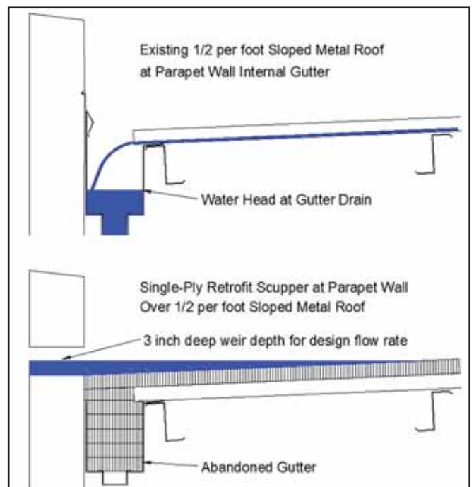
9. Concealed gutters are often covered in retrofit single-ply roofs.
