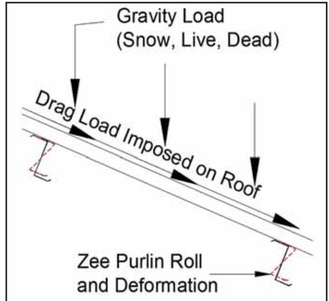
13. Drag load may result in purlin roll.
