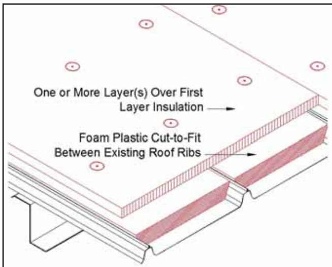
15. One example of single-ply roof retrofit insulation.
