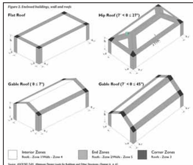
10. Wind uplift zones on varying roof slopes and configurations.
