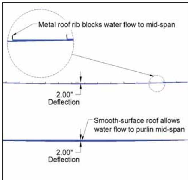
7. Comparison of water flow to purlin mid-span.
