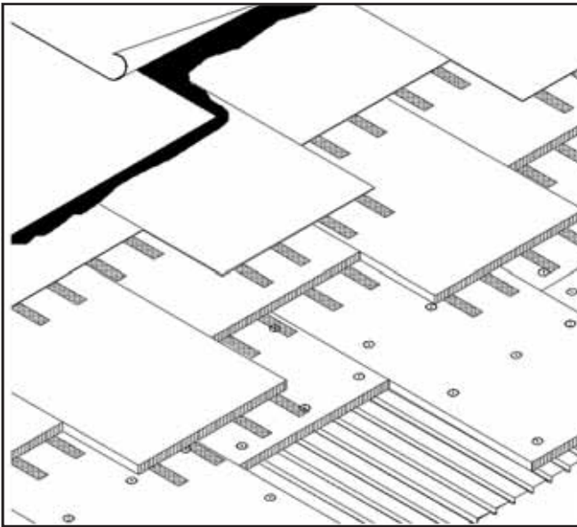
4. Example of steel deck and insulated single-ply roof.
