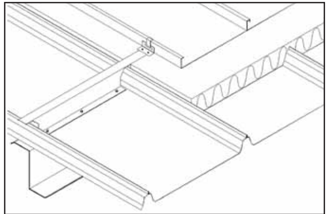
1. Example of a metal over metal retrofit assembly.
