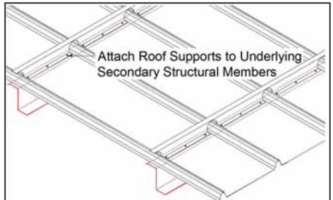
11. New roof supports attached through existing roof.
